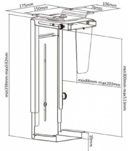
Technical drawing
